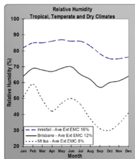
Climatic effects on timber floors
