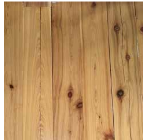
Edge bonding can result in wide irregularly spaced gaps at board edges and split boards.
