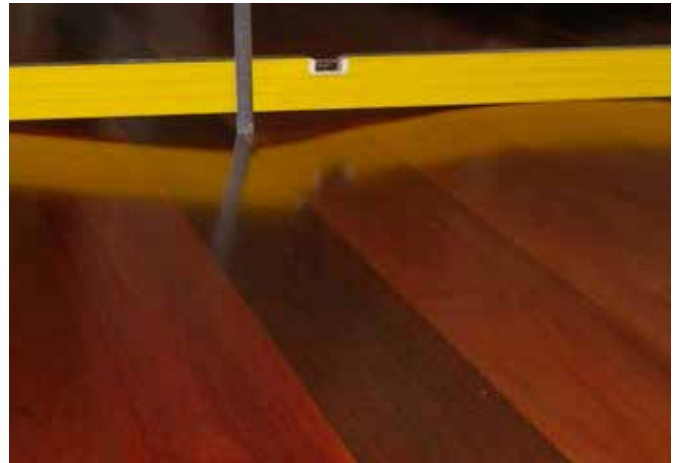
Buckling of the plywood subfloor off the joists.
