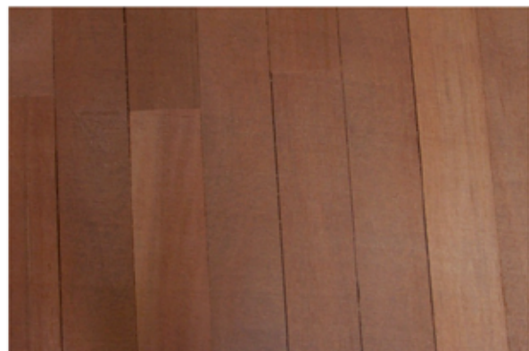
Wide gaps due to high moisture contents at the time of machining.
