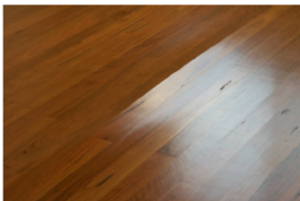
Tenting resulting from atmospheric moisture uptake.
