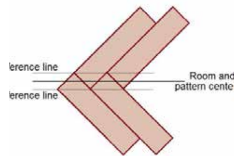
Center and reference lines with herringbone pattern
