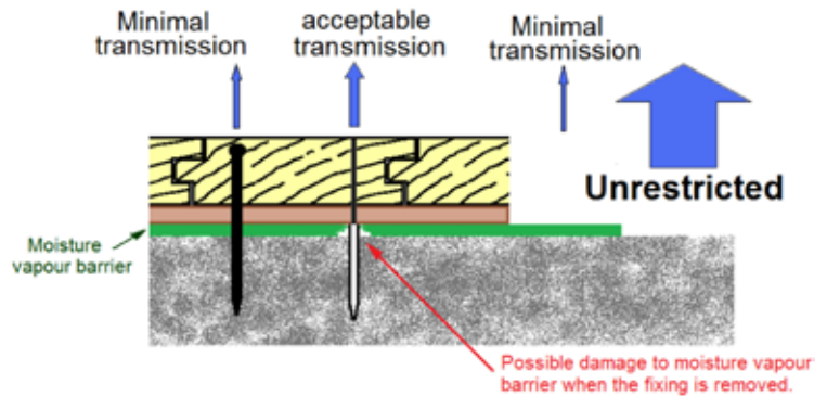
Effect of fixings through moisture vapour retarding barrier
