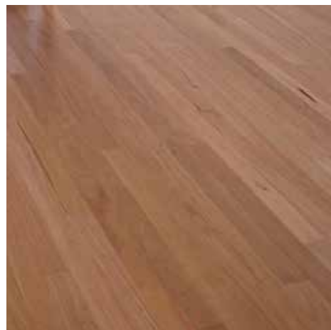
A select grade Blackbutt floor where the backsawn gum vein toward the top right exceeds grade limits but is acceptable within the floor.
