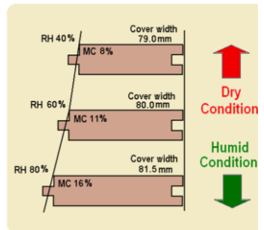
Cover width variation with changing relative humidity.
