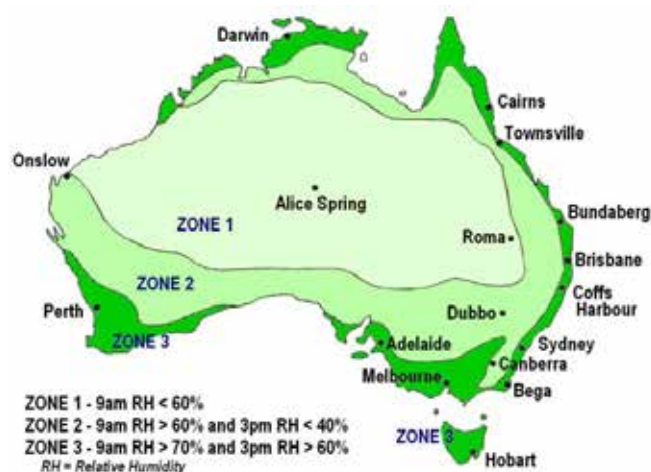
Source: NCC 2015 Vol 2 Figure 3.4.1.2
