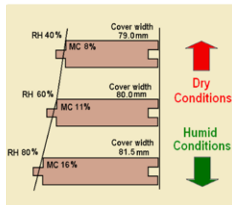
Indicative relationship between relative humidity, timber moisture content and board width.
