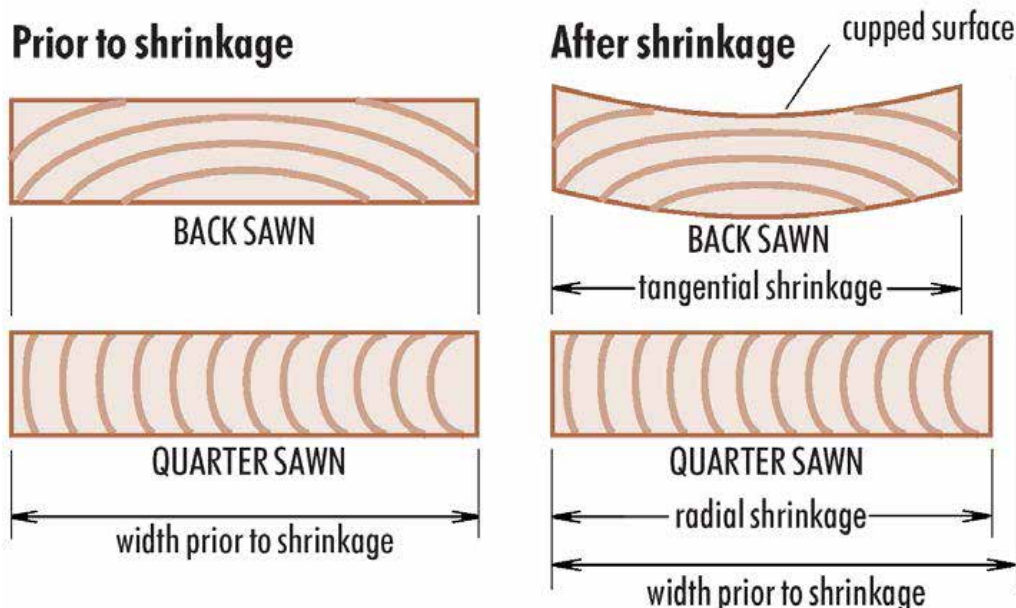
Backsawn and quartersawn floorboards.
